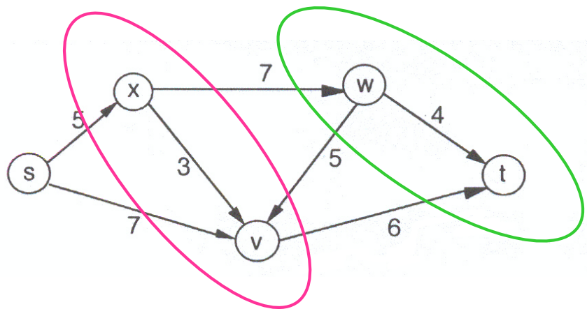
A 5-vertex capacitated network with source s and sink t .
