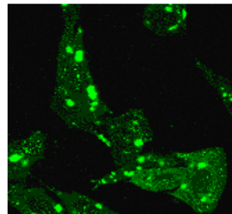
oGPCR-B, Induced
