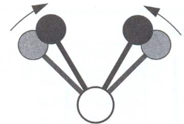
in-plane "scissoring"
