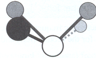
out-of-plane "twisting"
