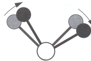
in-plane "rocking"
