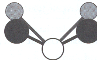
out-of-plane "wagging"
