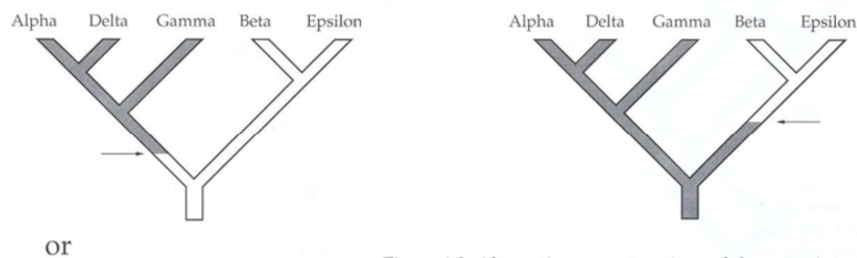
Figure 1.2: Alternative reconstructions of character 1 on the phylogeny of Figure 1.1. The white region of the tree is reconstructed as having state 0, the shaded region as having state 1. The two reconstructions each have one change of state. The changes of state are indicated by arrows.
