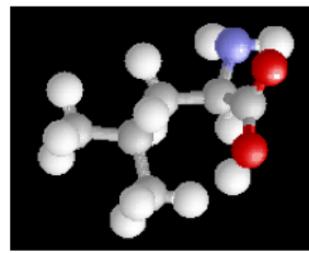
Leucine
