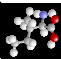
Isoleucine
