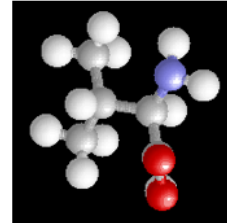
Valine
