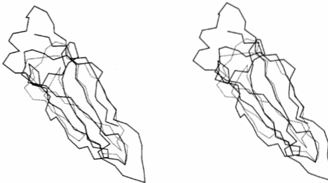
Fig. 2. Structure alignment of papD and CD4. Structural alignment and optimal superposition of papD protein (3DPA) and CD4 T-cell receptor (1CD4). The C ^{\alpha} -rmsd after optimal superposition is 1.5 Å for 41 aligned residues. PDB residue numbers of the aligned fragments follow. For 3DPA: 16–38, 85–94, 105–112. For 1CD4: 111–133, 154–163, 166–173. The alignment was generated using the Suppos algorithm.
