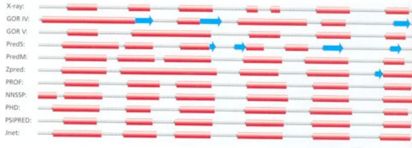
all \alpha protein
