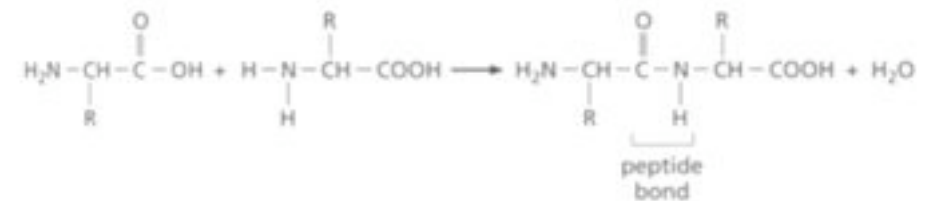
Figure 2.4 Peptide bond chemical structure bond that acids to m (B) illustra diagramm Alberts et al the Cell, 41 Science, 20
