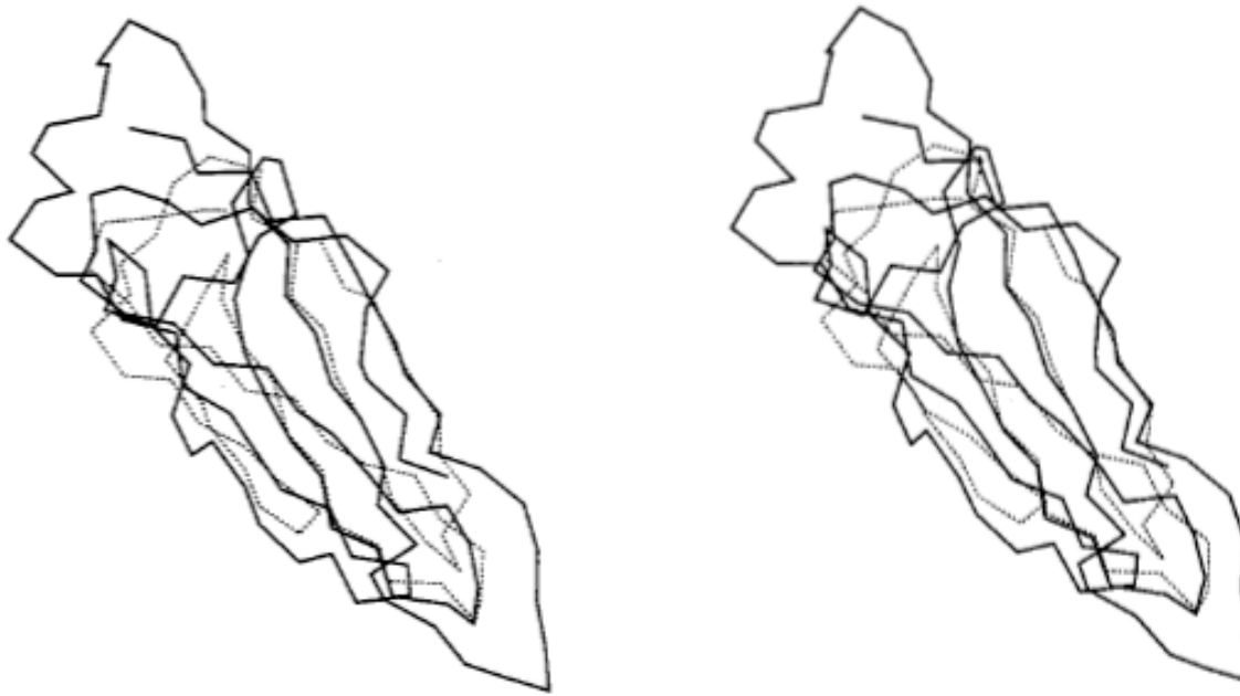
Fig. 2. Structure alignment of papD and CD4. Structural alignment and optimal superposition of papD protein (3DPA) and CD4 T-cell receptor (1CD4). The C \alpha -rmsd after optimal superposition is 1.5 Å for 41 aligned residues. PDB residue numbers of the aligned fragments follow. For 3DPA: 16–38, 85–94, 105–112. For 1CD4: 111–133, 154–163, 166–173. The alignment was generated using the Suppos algorithm.
